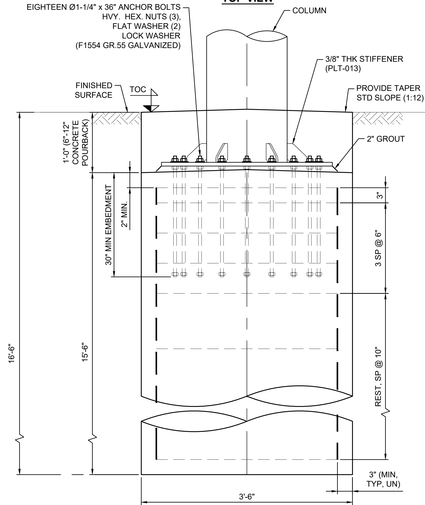
FOOTING TYPE C Ø 3'-6" X 15'-6" T D (RBP-RECESSED BASE PLATE) USE FOR NON-CONSTRAINED CASES
