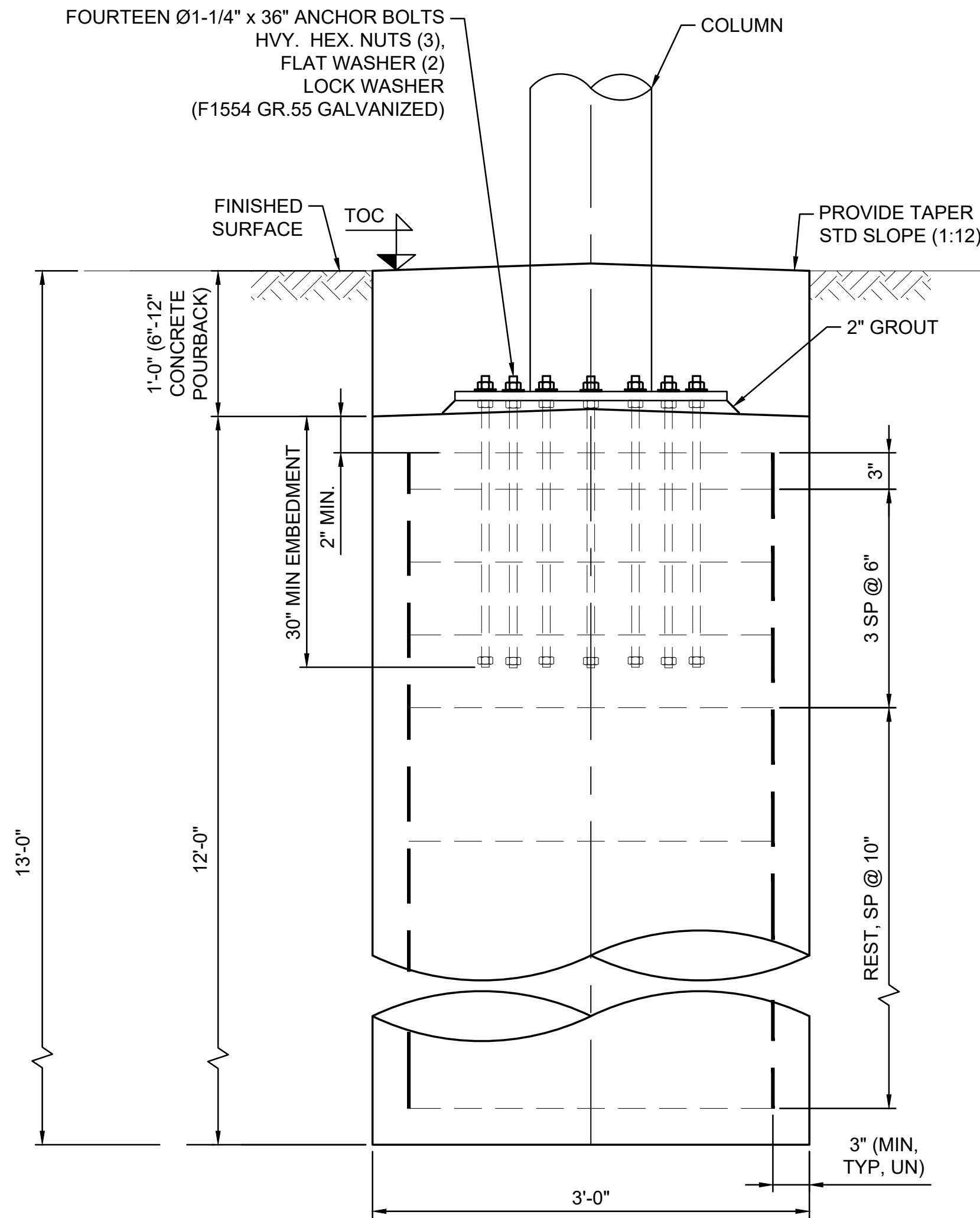
FOOTING TYPE A Ø3'-0" X 12'-0" T D (RBP-RECESSED BASE PLATE) USE FOR NON-CONSTRAINED CASES
