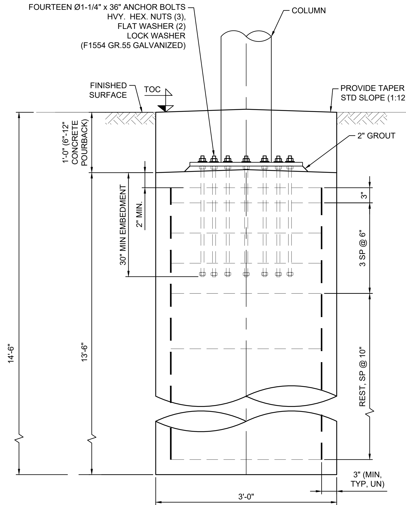
FOOTING TYPE B Ø3'-0" X 13'-6" T D (RBP-RECESSED BASE PLATE) USE FOR NON-CONSTRAINED CASES
