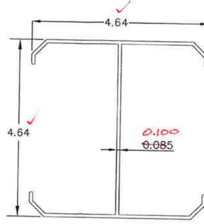
G10HA - ALUMINUM (6063-T6) POST INSERT
