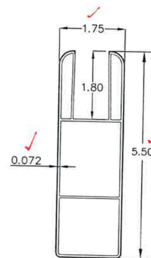
F37C - 1 1/4" x 5 1/2" GORILLA POCKET RAIL (DOUBLE NOTCHED)
