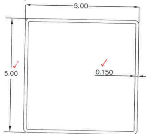
F10C - 5"x 5"x 9' POST
