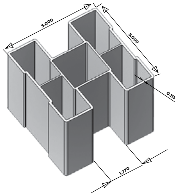
5" X 5" GORILLA® H-POST
