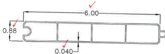
F54G - GORILLA T&G BOARD
