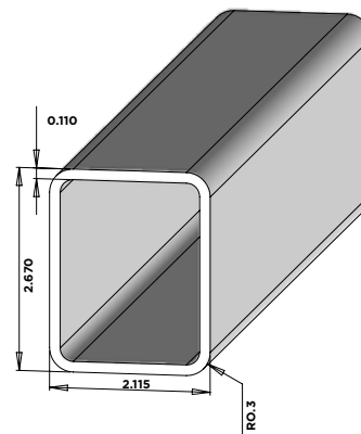
2-1/8" X 2-3/4" STANDARD RAIL
