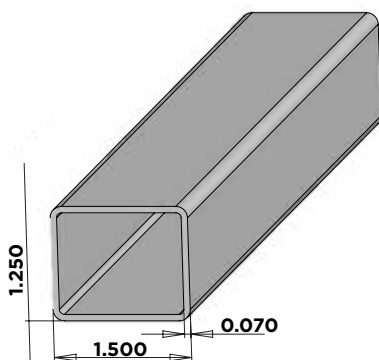
1-1/4" X 1-1/2" STANDARD PICKETS
