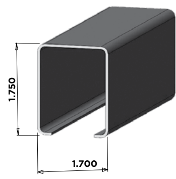
2" STEEL INSERT - 2" POCKET RAIL
