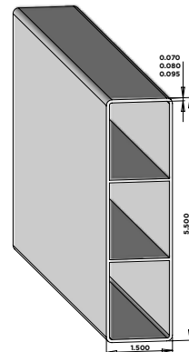
1-1/2" X 5-1/2" RIBBED RAIL
